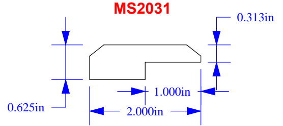
Square Nose Reducer
